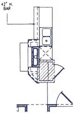
STANDARD FIREPLACE
