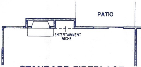
STANDARD FIREPLACE W/ OPTIONAL ENTERTAINMENT NICHE
